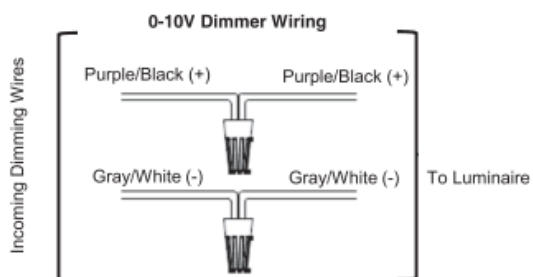
Wiring Diagram 2
