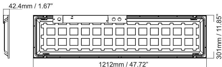
PLB2 1' x 4' Dimensions mm | 1212 (L) x 301 (W) x 42.4 (H) inch | 47.72 (L) x 11.85 (W) x 1.67 (H)
