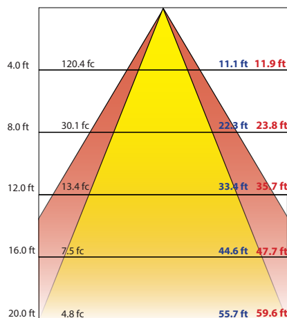
Illuminance at distance
